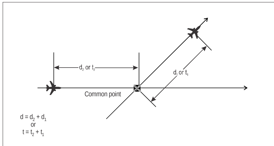
Figure 5-34. Calculation of longitudinal distance/time between aircraft — opposite sides of the common point (see 5.4.2.9.5 b))
