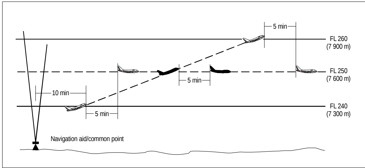
Figure 5-18A. Five-minute separation between aircraft climbing and on same track (see 5.4.2.2.1 c) 2))
